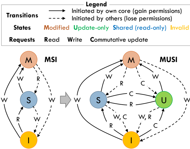
Figure 4: State-transition diagrams of MSI and MUSI protocols. For clarity, diagrams omit actions that do not cause a state transition (e.g., R requests in S).
